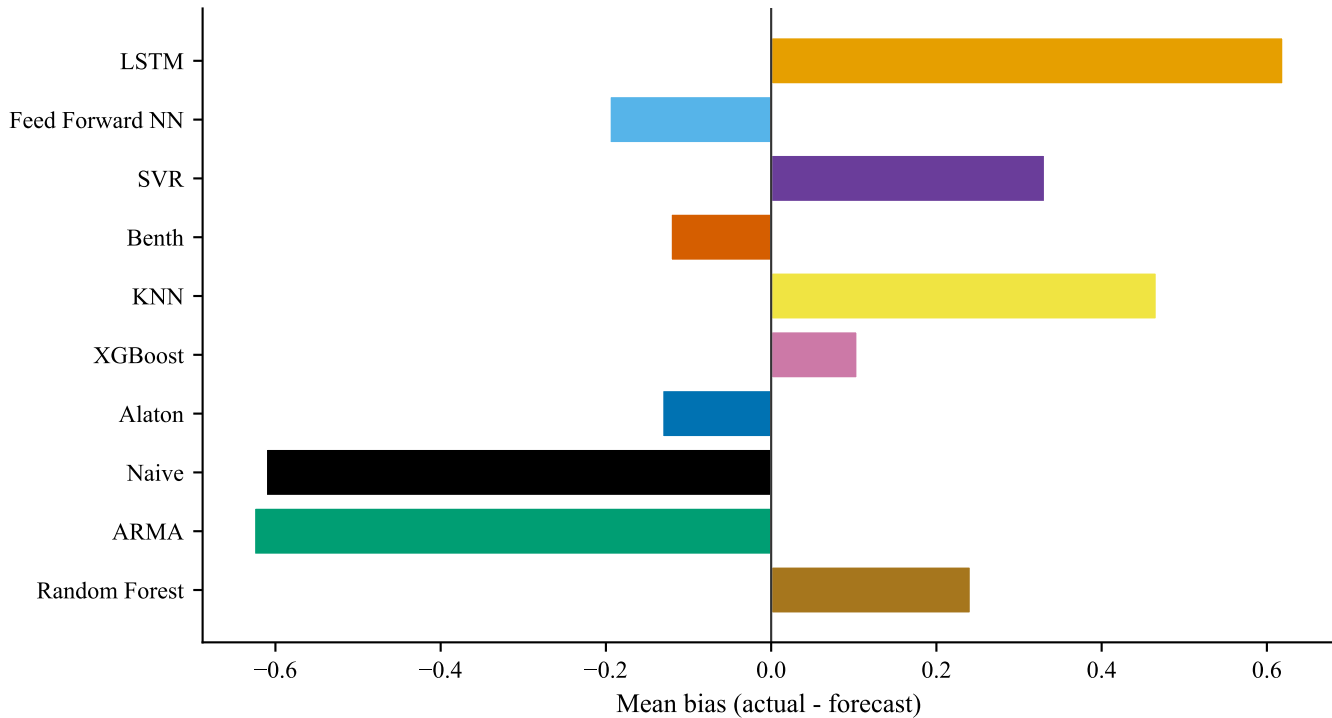
Average Forecast Bias by Model
